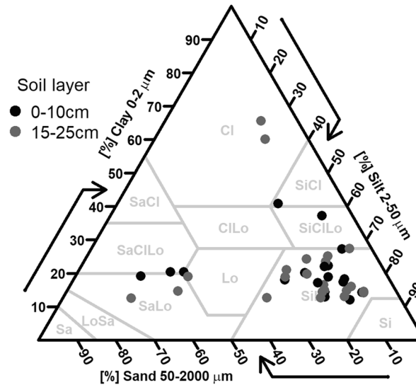
Fig. 1 Texture of the undisturbed soils studied according to the USDA classification (US Department of Agriculture classification system) and European classification (Hartshorne and Dicken 1935). The arrows along the axes of the soil texture triangle indicate the directions to assess the percentages of sand, silt, and clay
