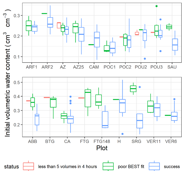
Fig. 6 Initial volumetric water content ( n=417 ) per plot and success rate of water infiltration measurement with the Beerkan method (less than 5 water volumes in 4 h=failure of in situ measurements) and of simulation with the BEST methods (poor BEST fit=relative error and bias of the BEST fits too high)
